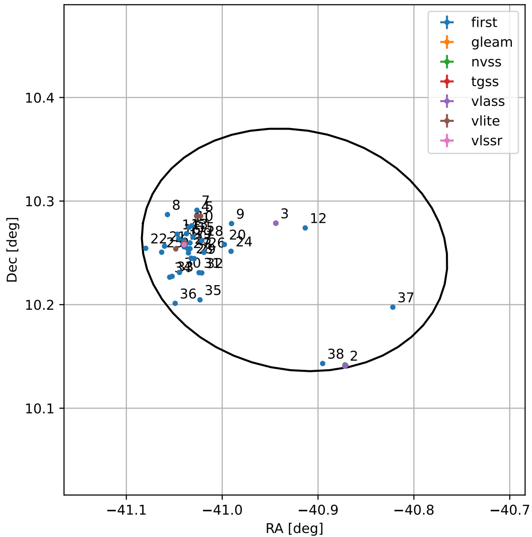
4FGL J2116.3+1015
