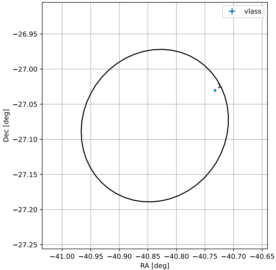
4FGL J2116.6-2704
