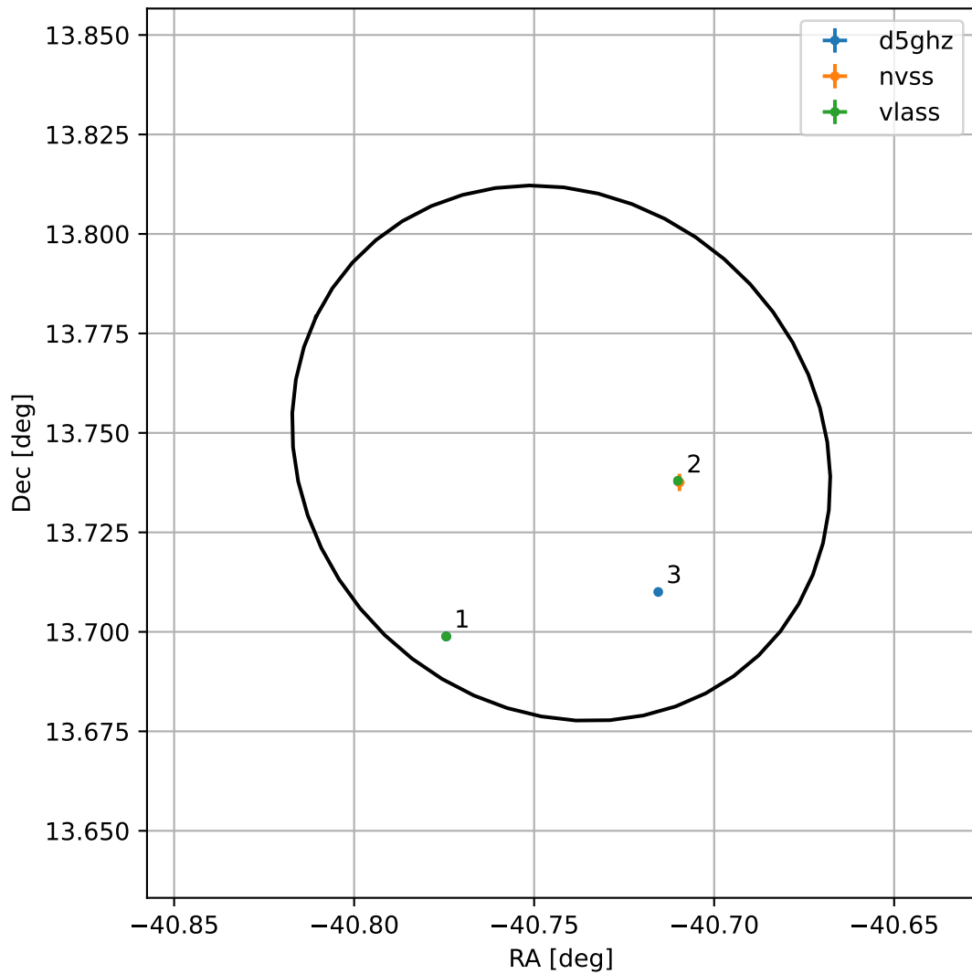
4FGL J2117.0+1344
