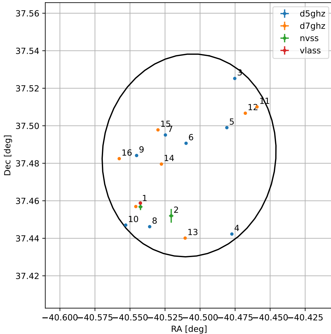
4FGL J2117.9+3729
