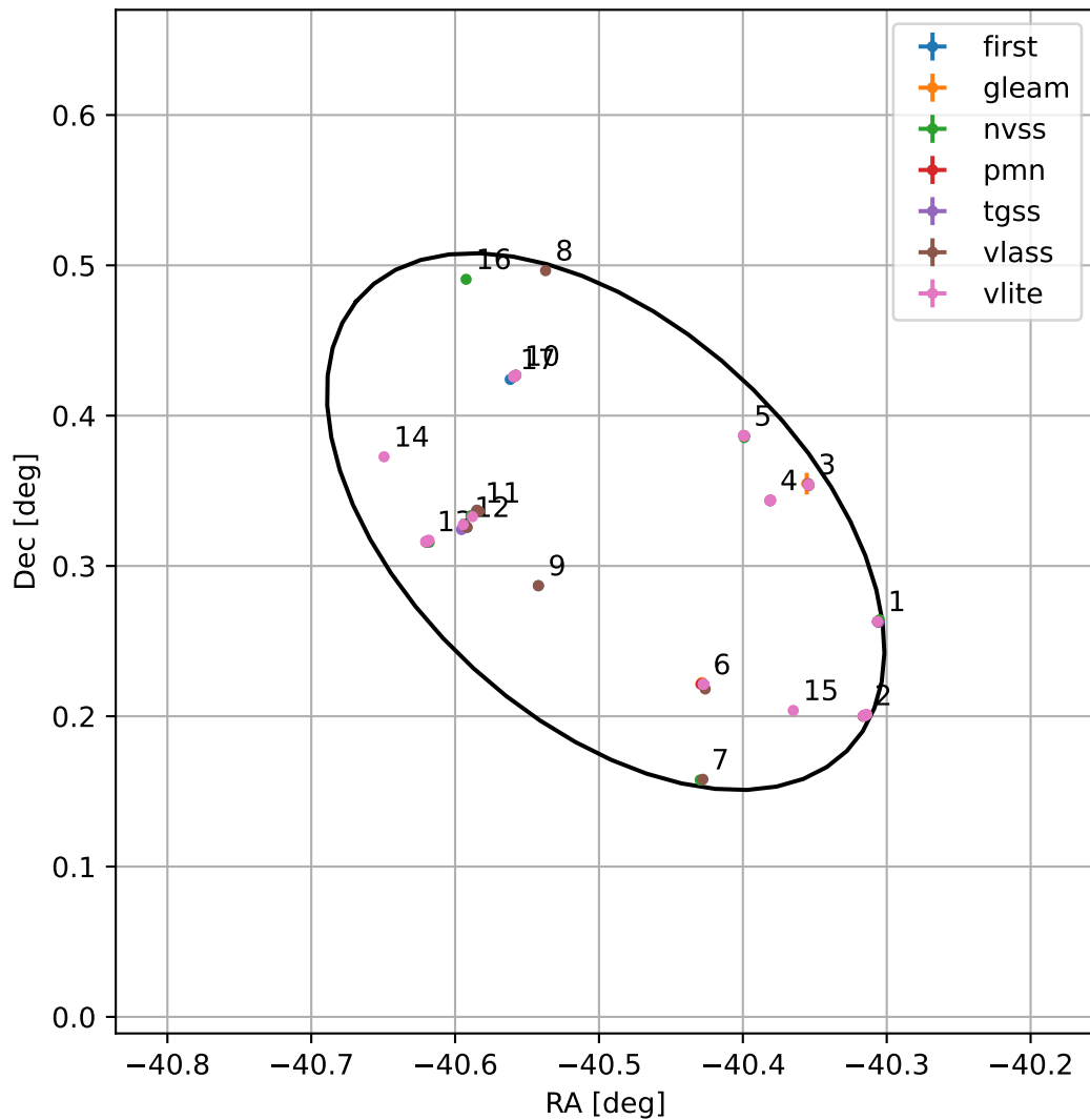
4FGL J2118.0+0019
