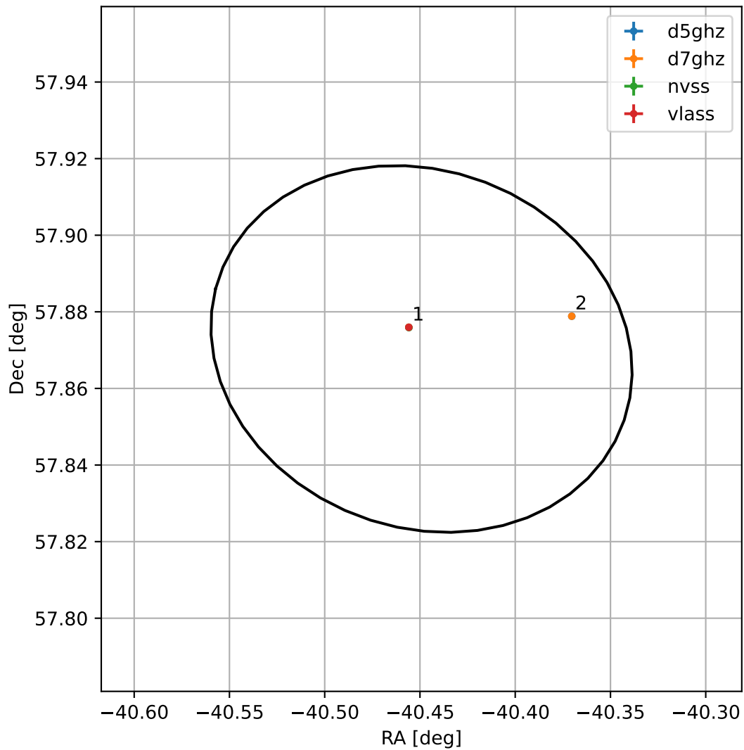
4FGL J2118.2+5752
