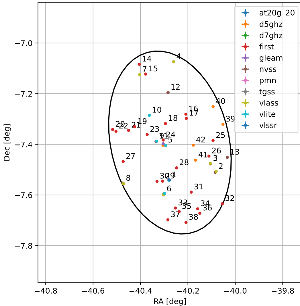
4FGL J2118.8-0723
