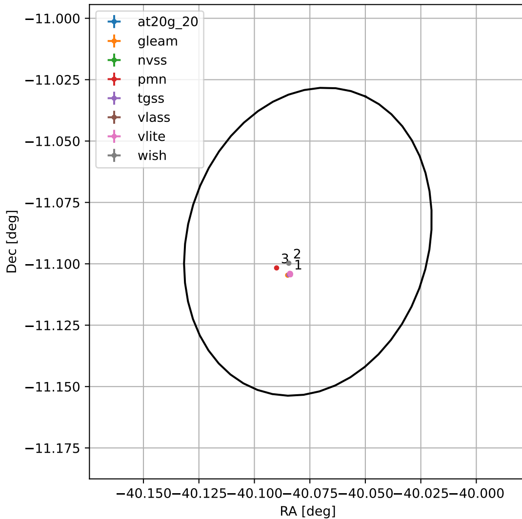
4FGL J2119.6-1105
