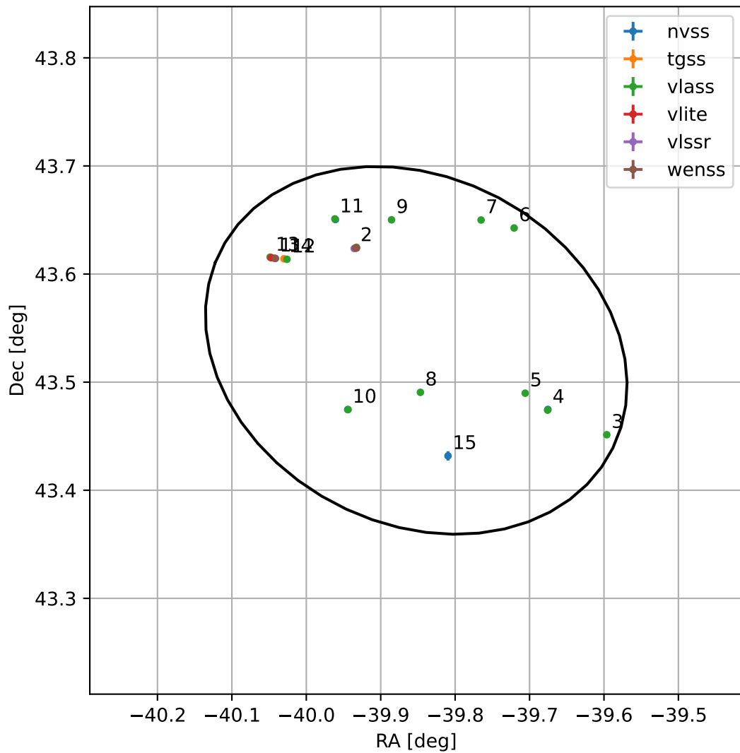
4FGL J2120.5+4331
