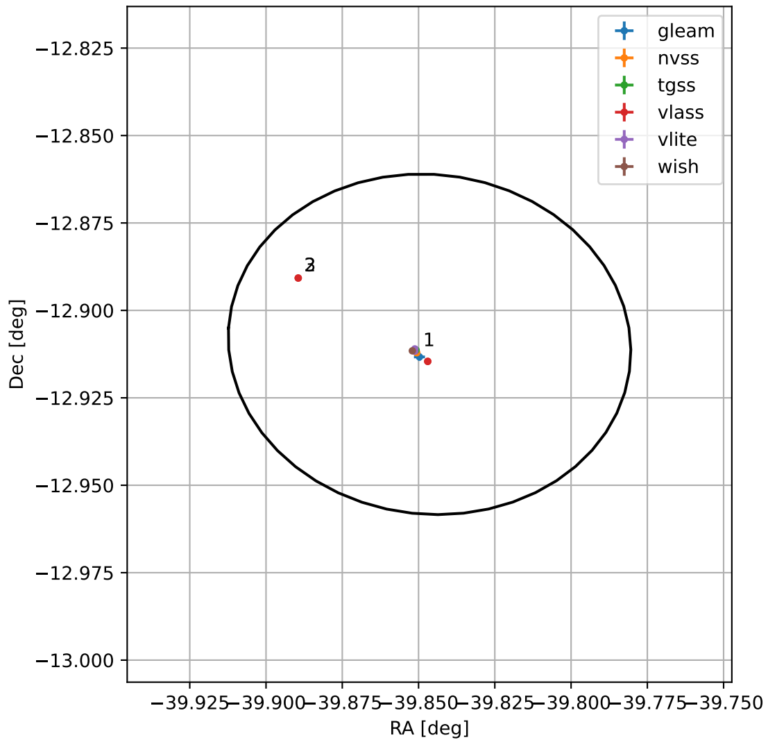
4FGL J2120.6-1254
