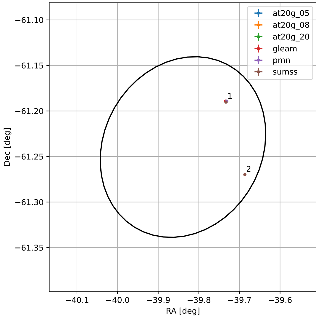
4FGL J2120.6-6114
