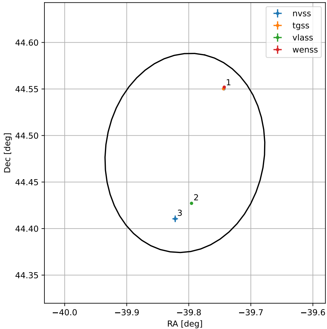
4FGL J2120.7+4428
