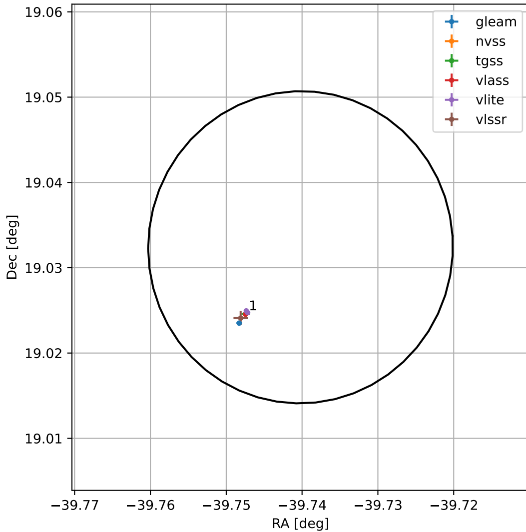
4FGL J2121.0+1901
