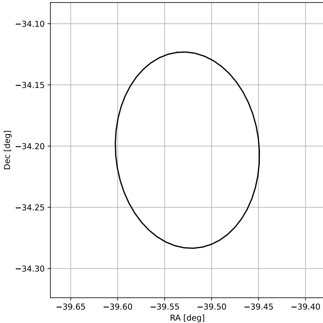
4FGL J2121.8-3412
