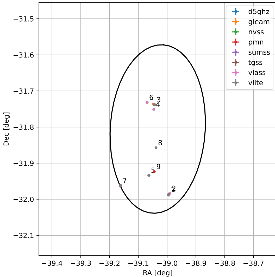
4FGL J2123.8-3148
