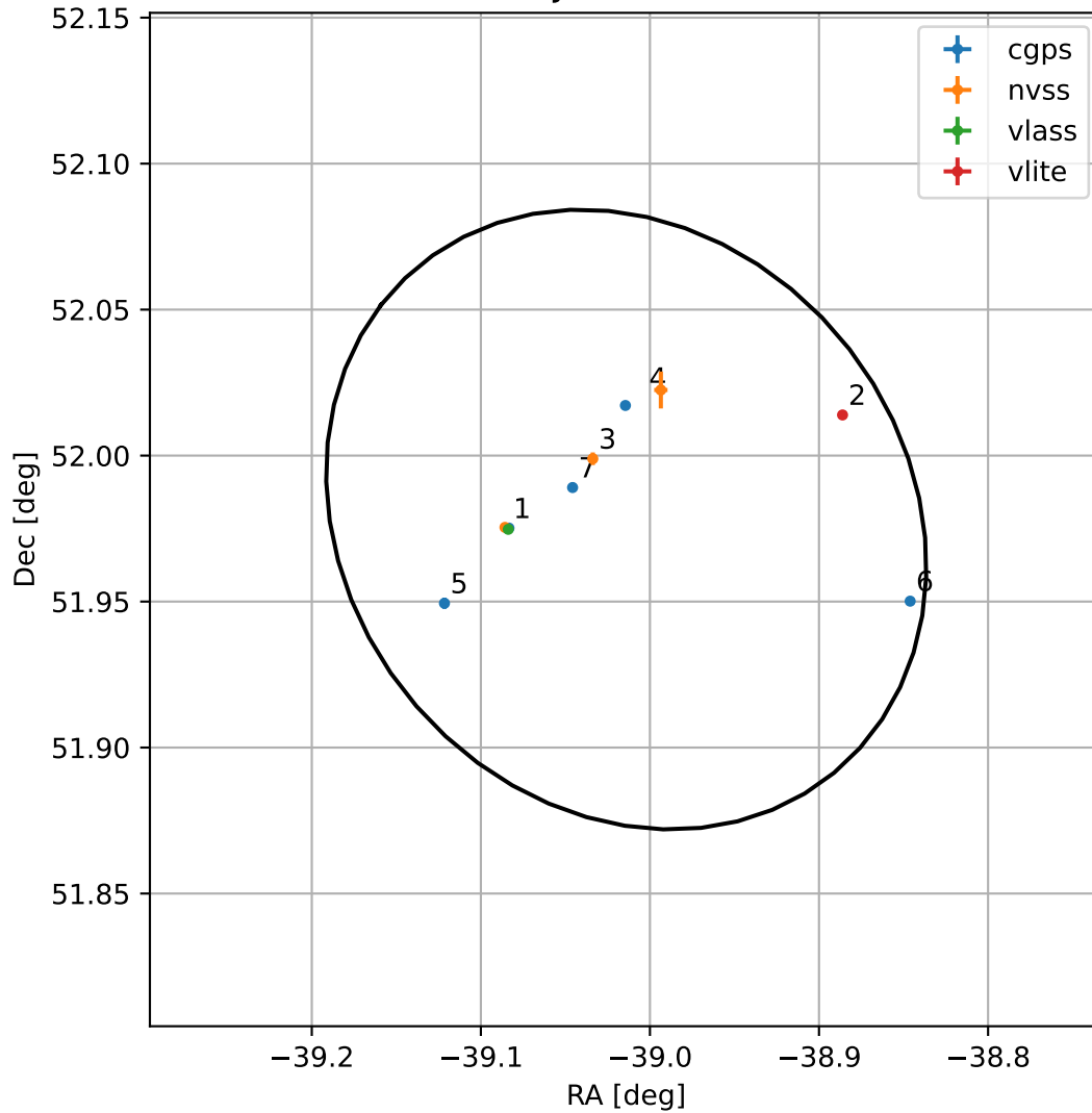
4FGL J2123.9+5158
