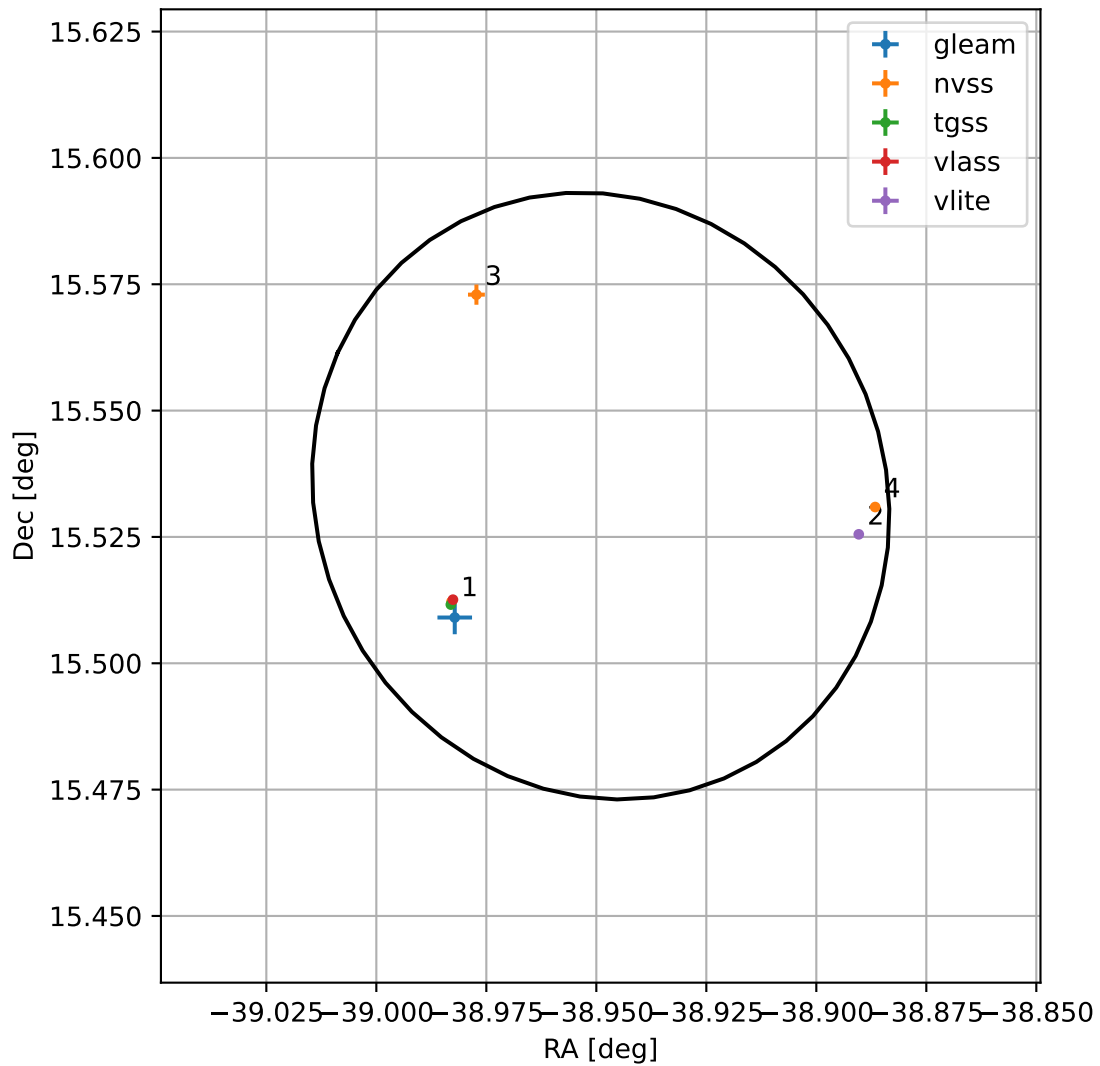
4FGL J2124.2+1531
