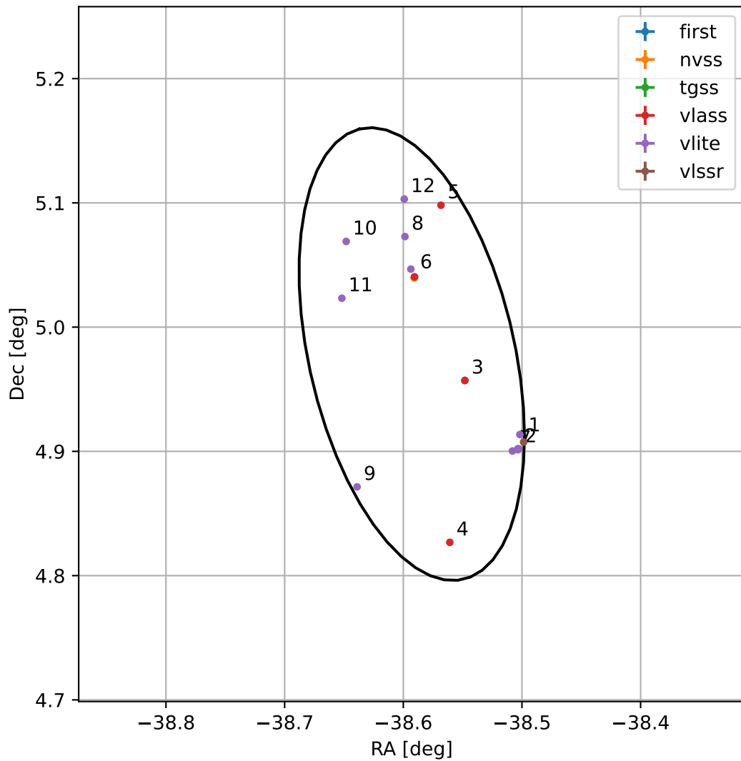
4FGL J2125.6+0458
