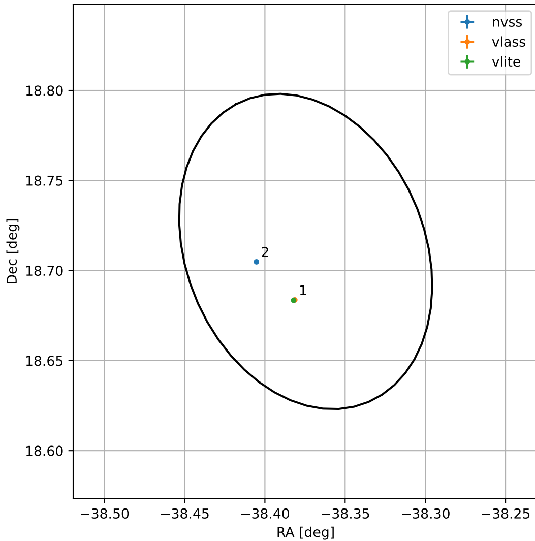
4FGL J2126.5+1842
