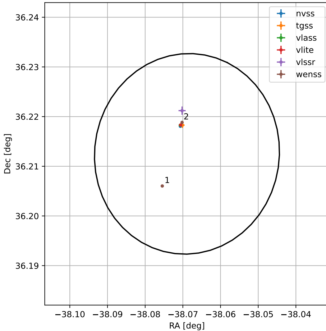
4FGL J2127.7+3612
