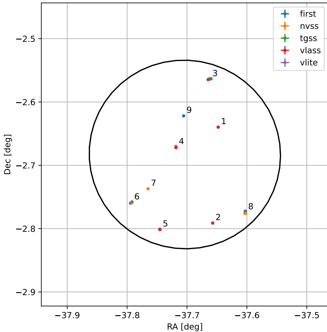
4FGL J2129.1-0240
