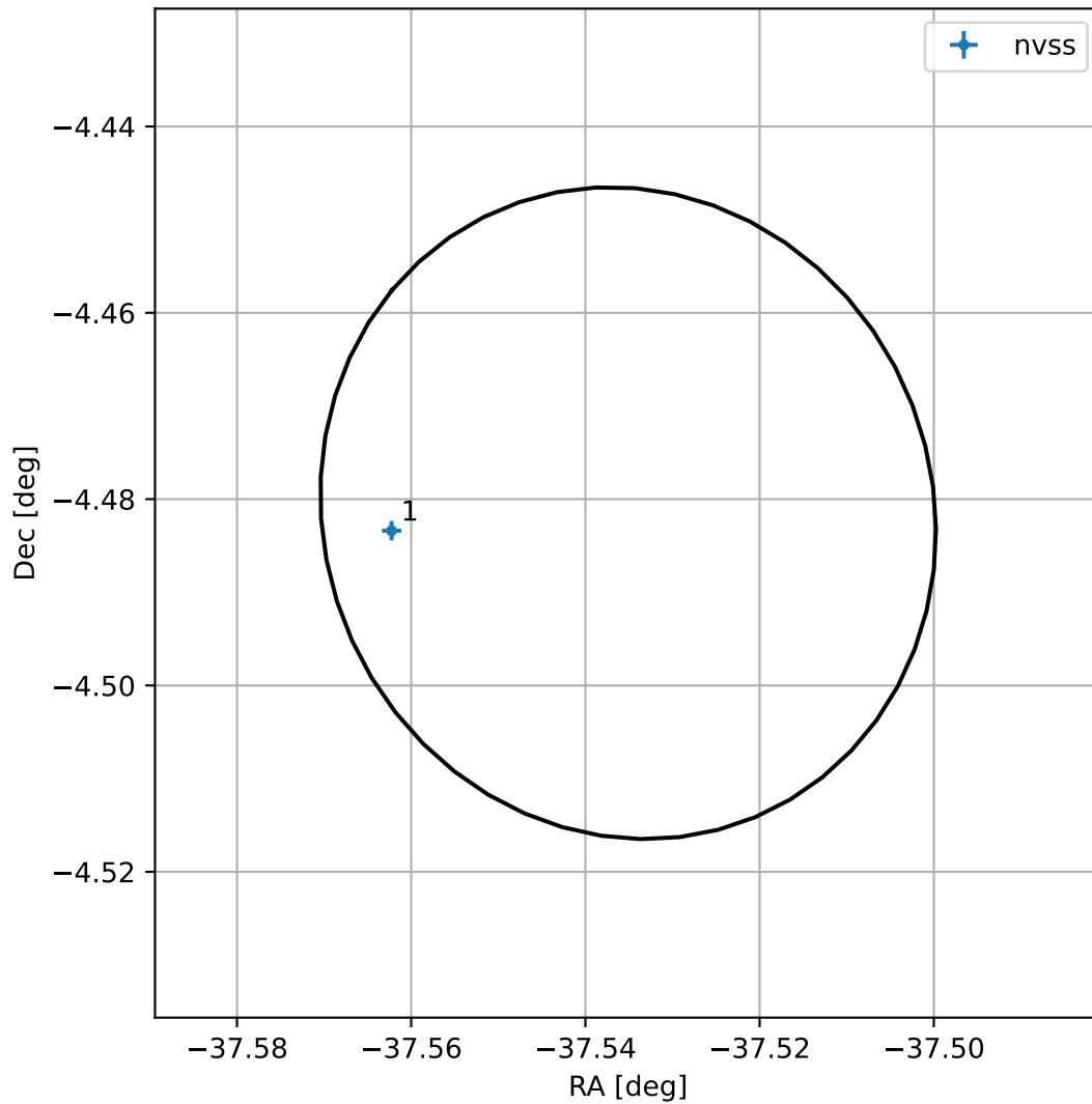
4FGL J2129.8-0428
