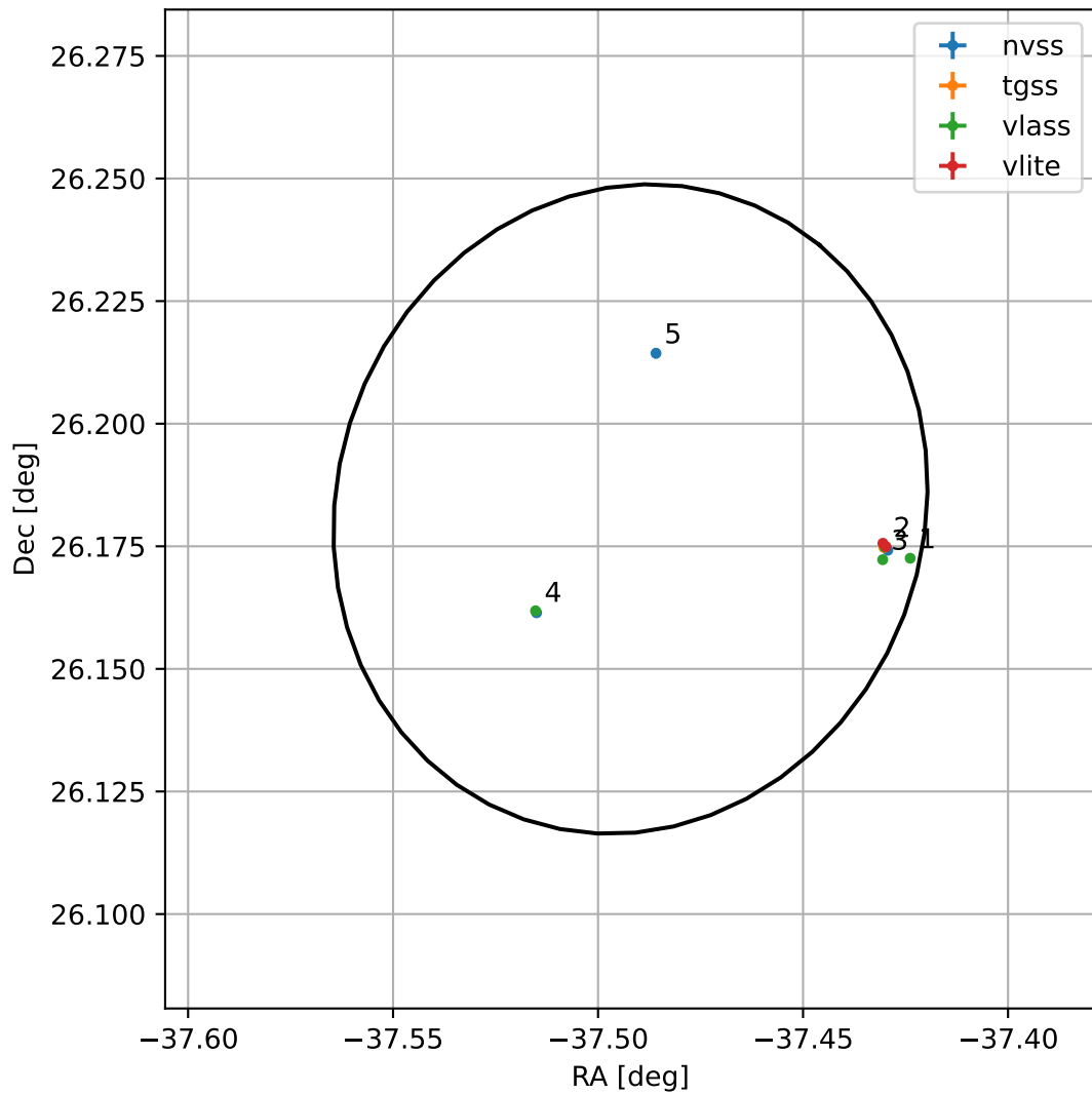
4FGL J2130.0+2610
