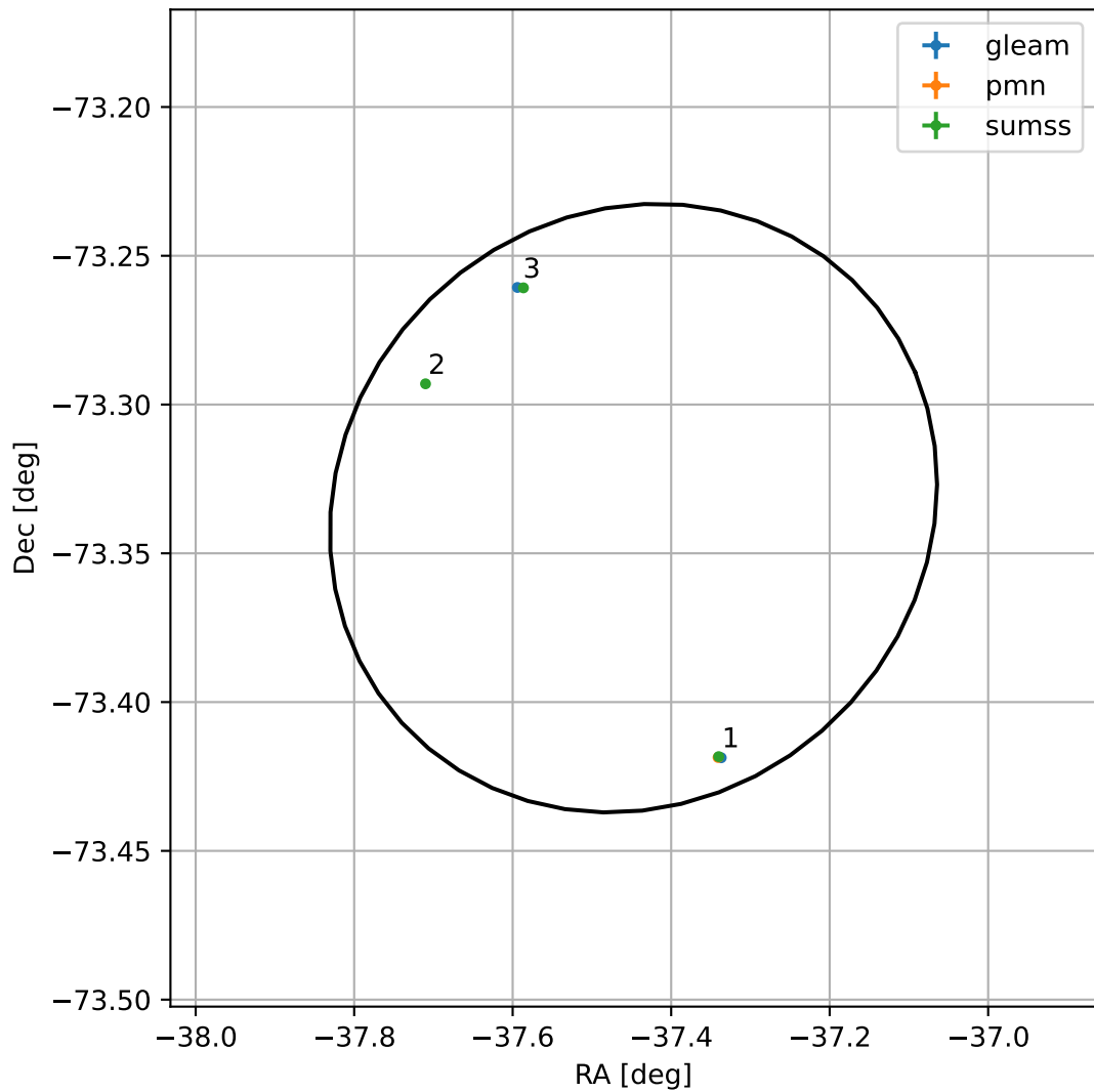
4FGL J2130.2-7320
