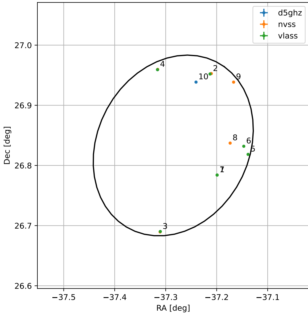
4FGL J2130.8+2649
