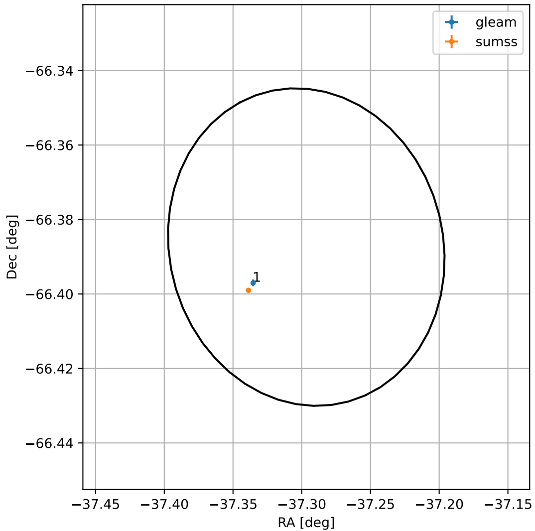
4FGL J2130.8-6623
