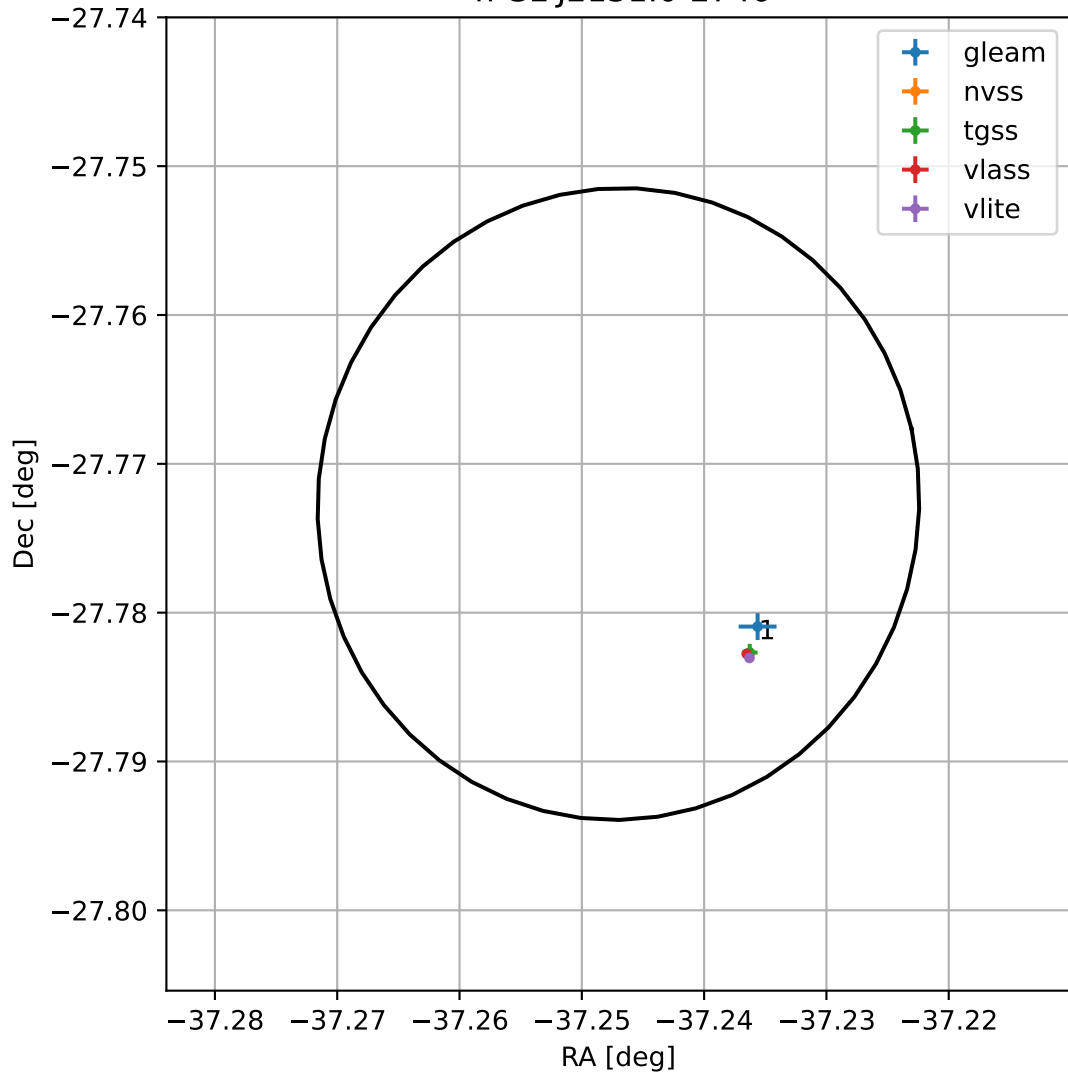
4FGL J2131.0-2746
