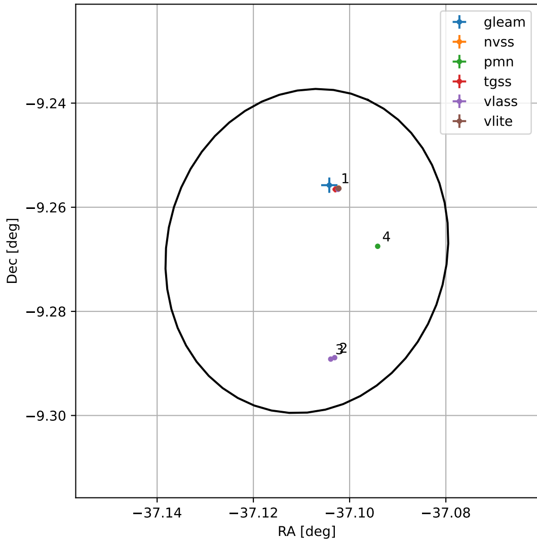
4FGL J2131.5-0916
