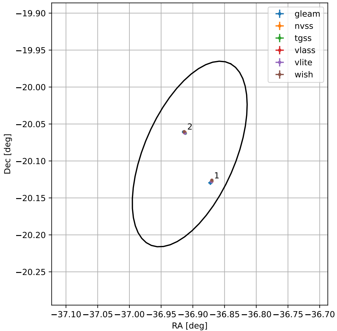
4FGL J2132.3-2005
