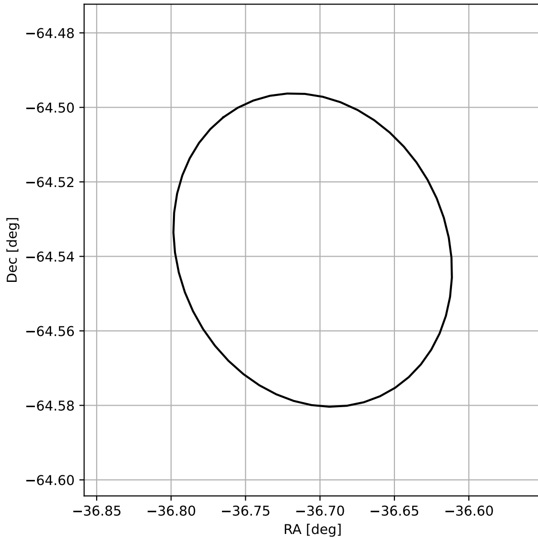
4FGL J2133.1-6432
