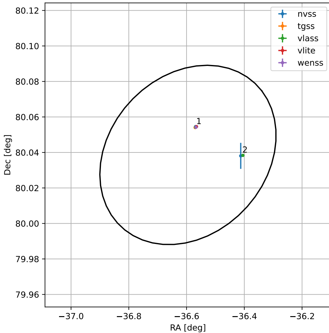
4FGL J2133.6+8002
