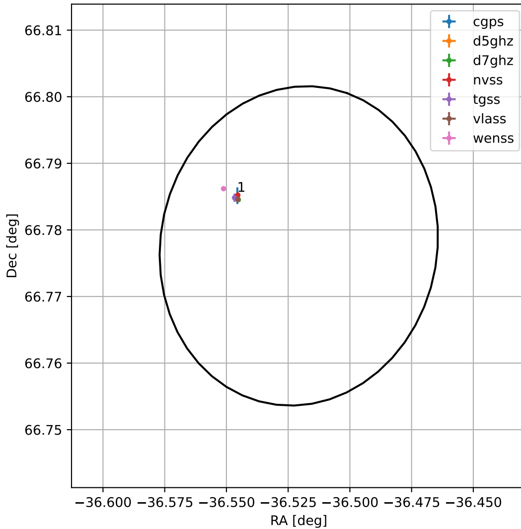
4FGL J2133.9+6646
