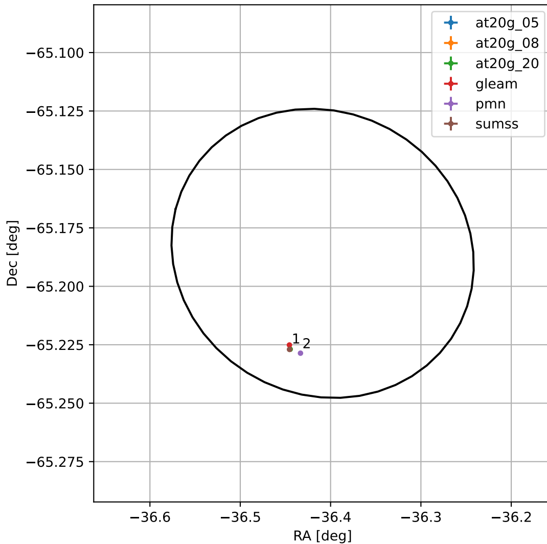
4FGL J2134.3-6511
