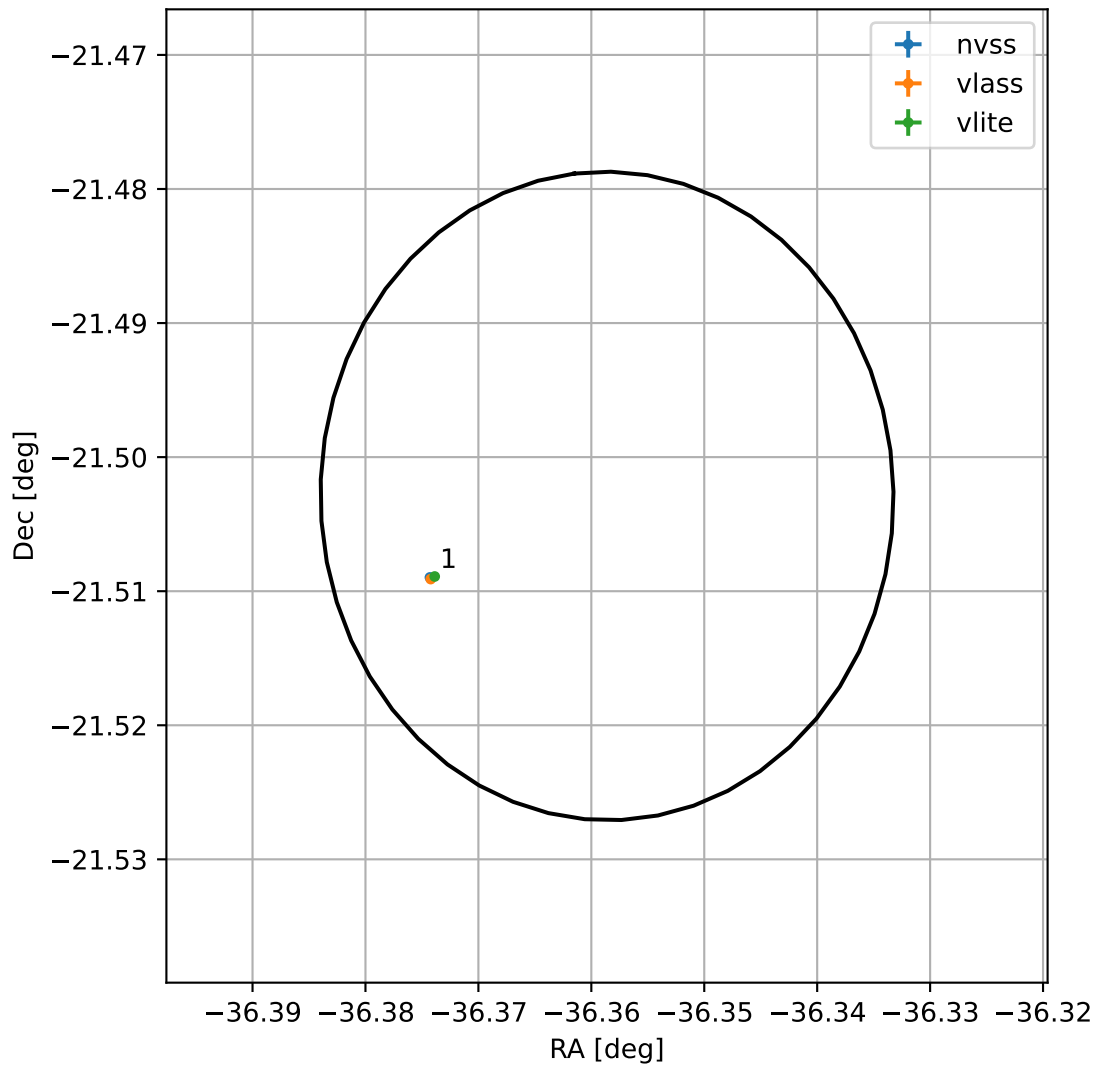
4FGL J2134.5-2130
