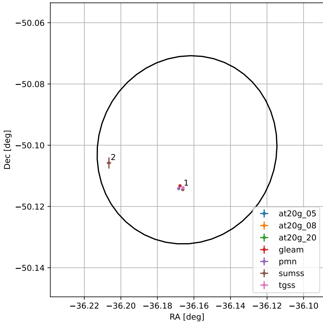
4FGL J2135.3-5006
