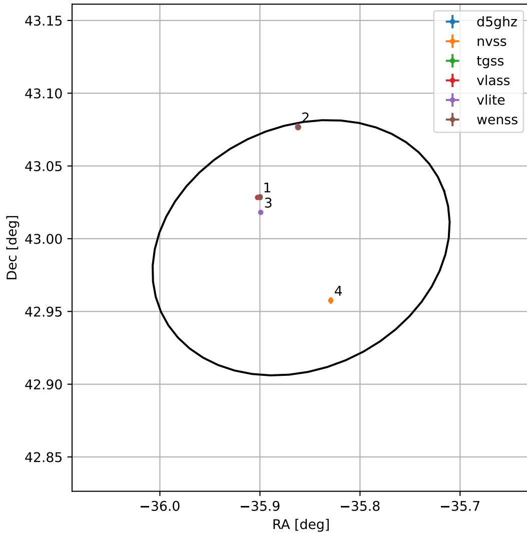
4FGL J2136.5+4259
