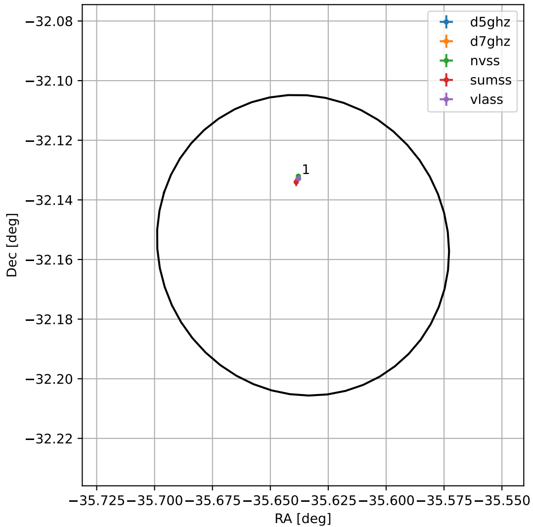
4FGL J2137.4-3209
