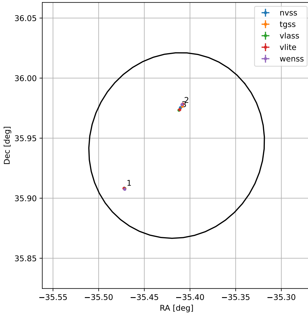
4FGL J2138.3+3556
