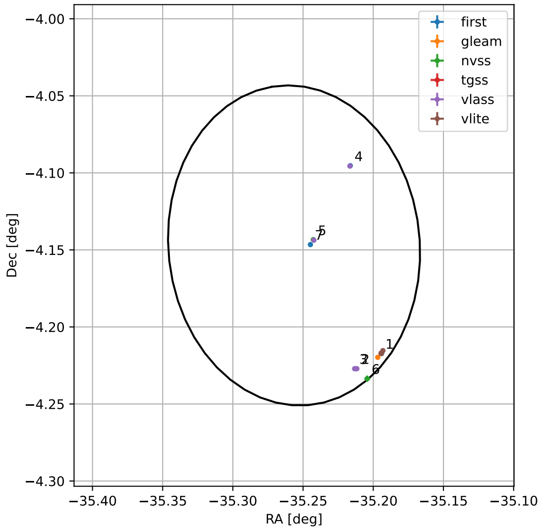
4FGL J2138.9-0408
