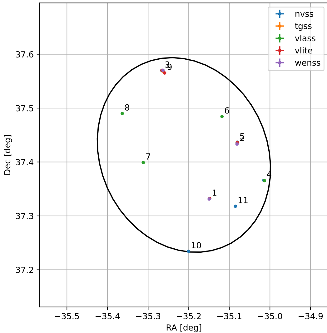
4FGL J2139.1+3724
