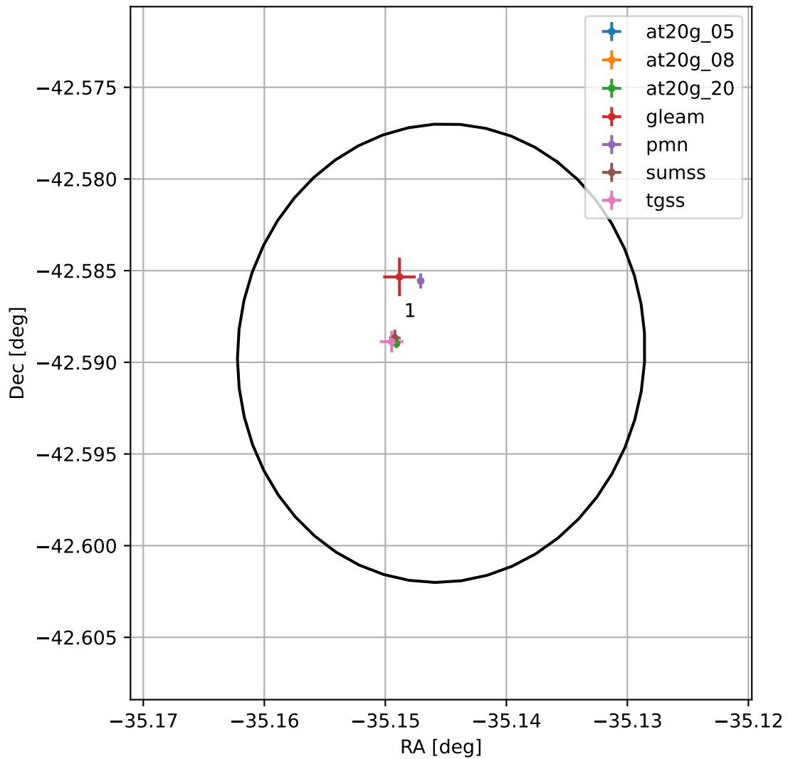
4FGL J2139.4-4235
