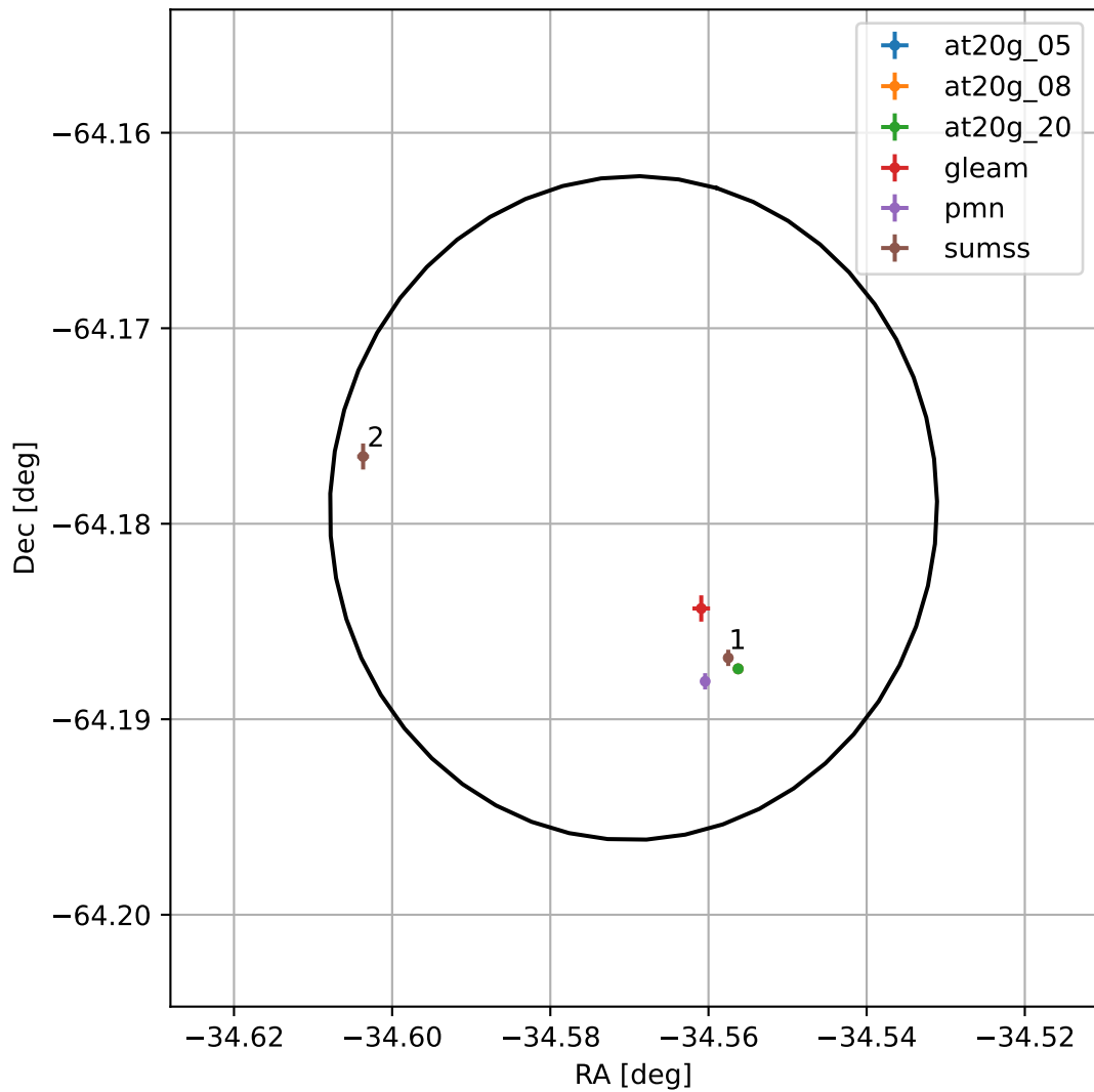
4FGL J2141.7-6410
