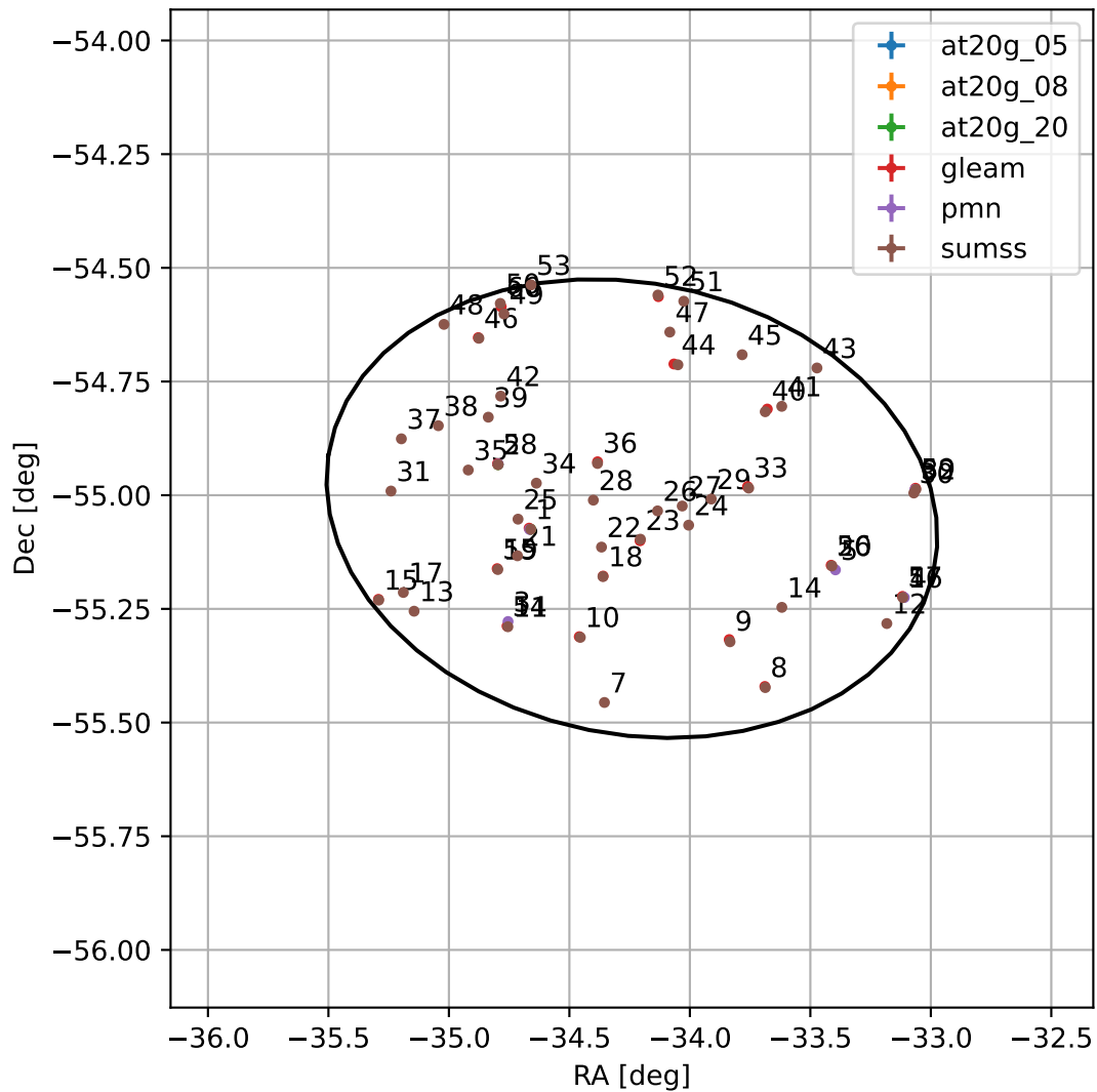
4FGL J2143.0-5501
