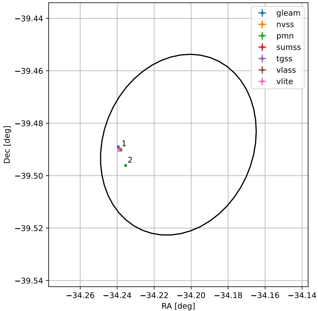
4FGL J2143.1-3929
