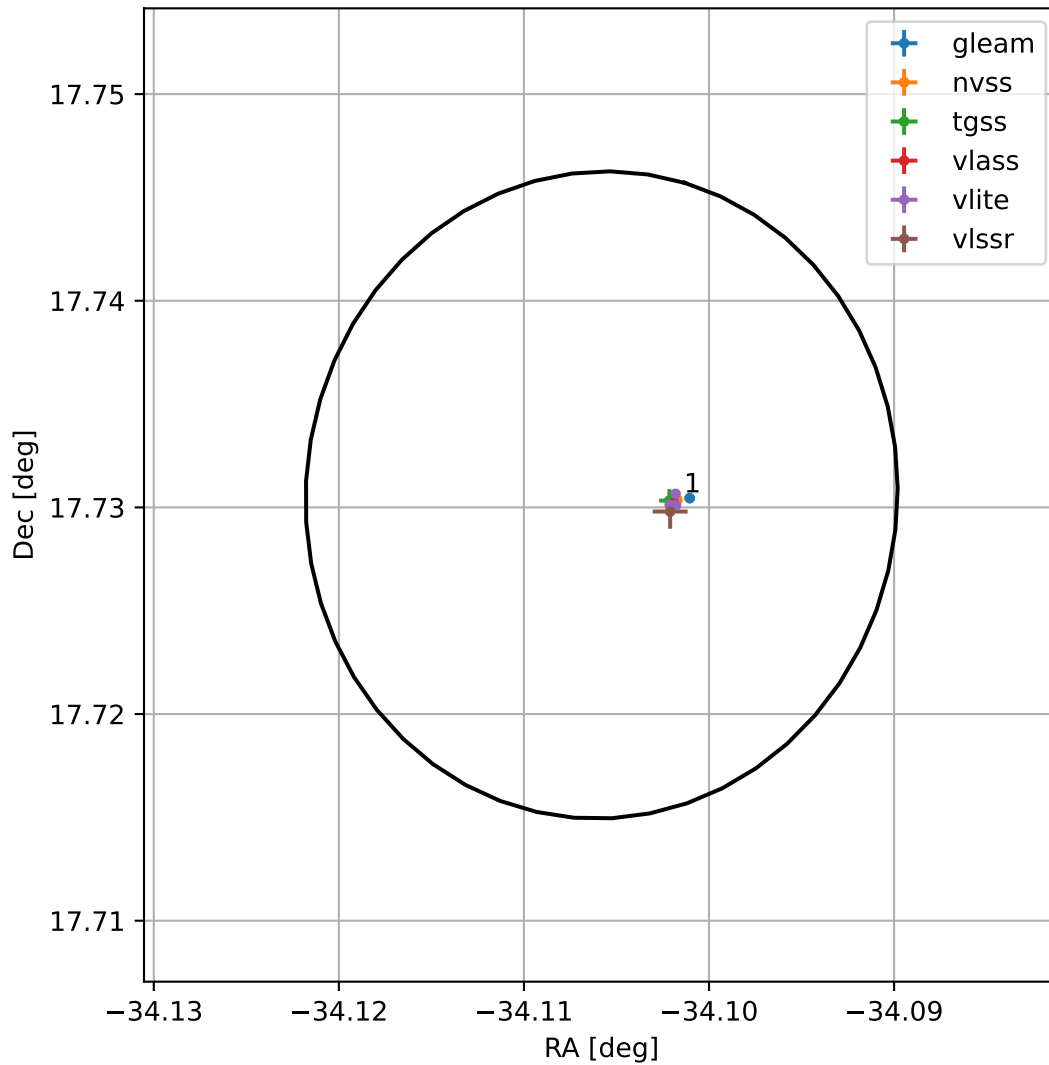
4FGL J2143.5+1743
