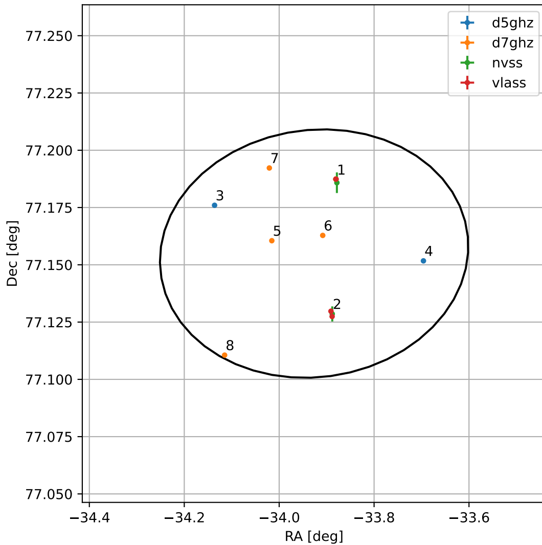
4FGL J2144.2+7709
