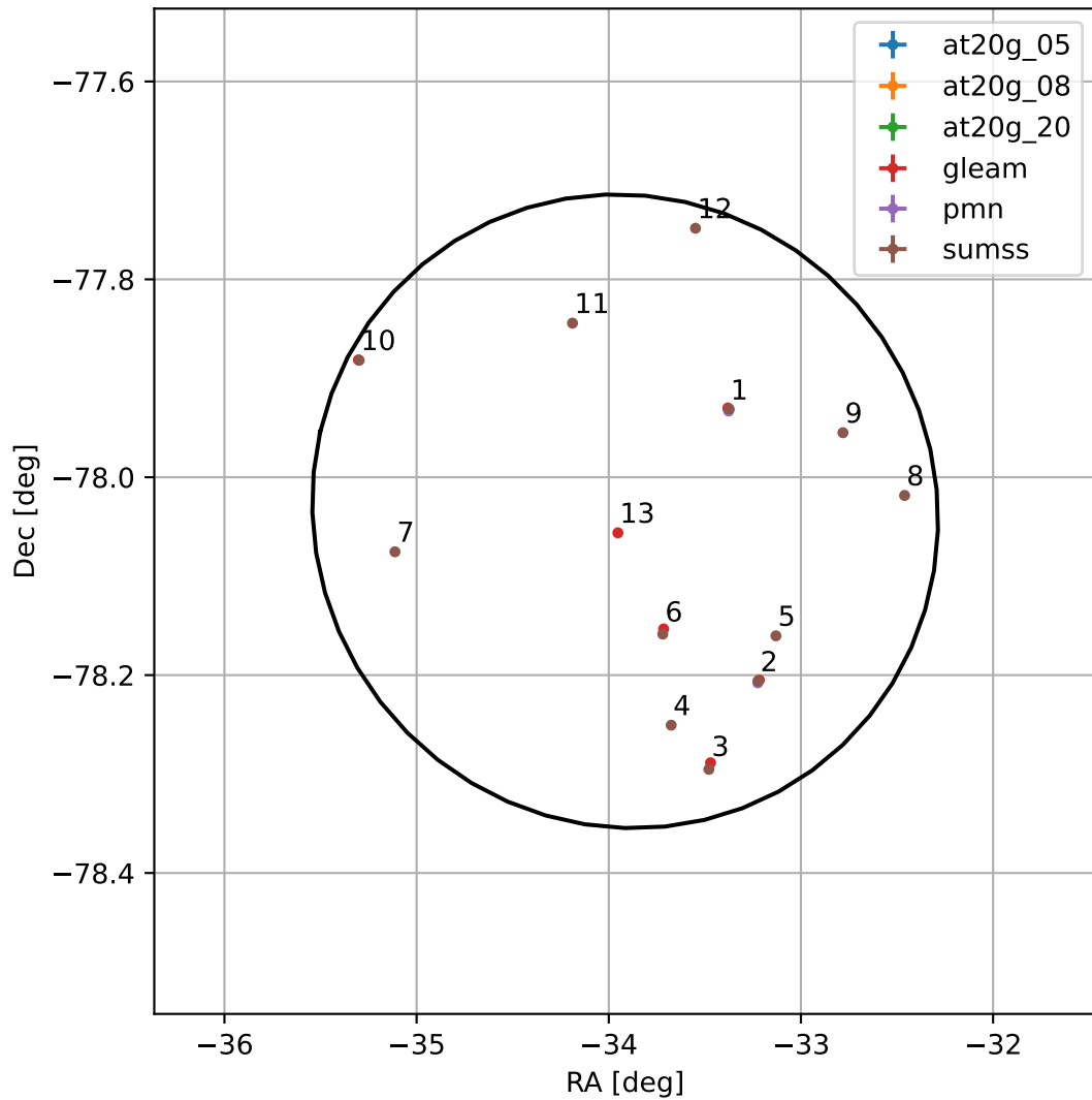
4FGL J2144.3-7802
