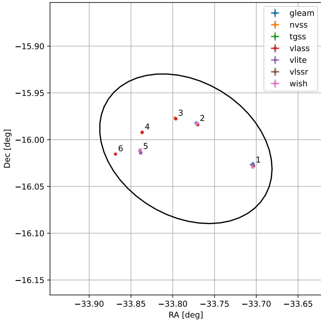
4FGL J2144.8-1600
