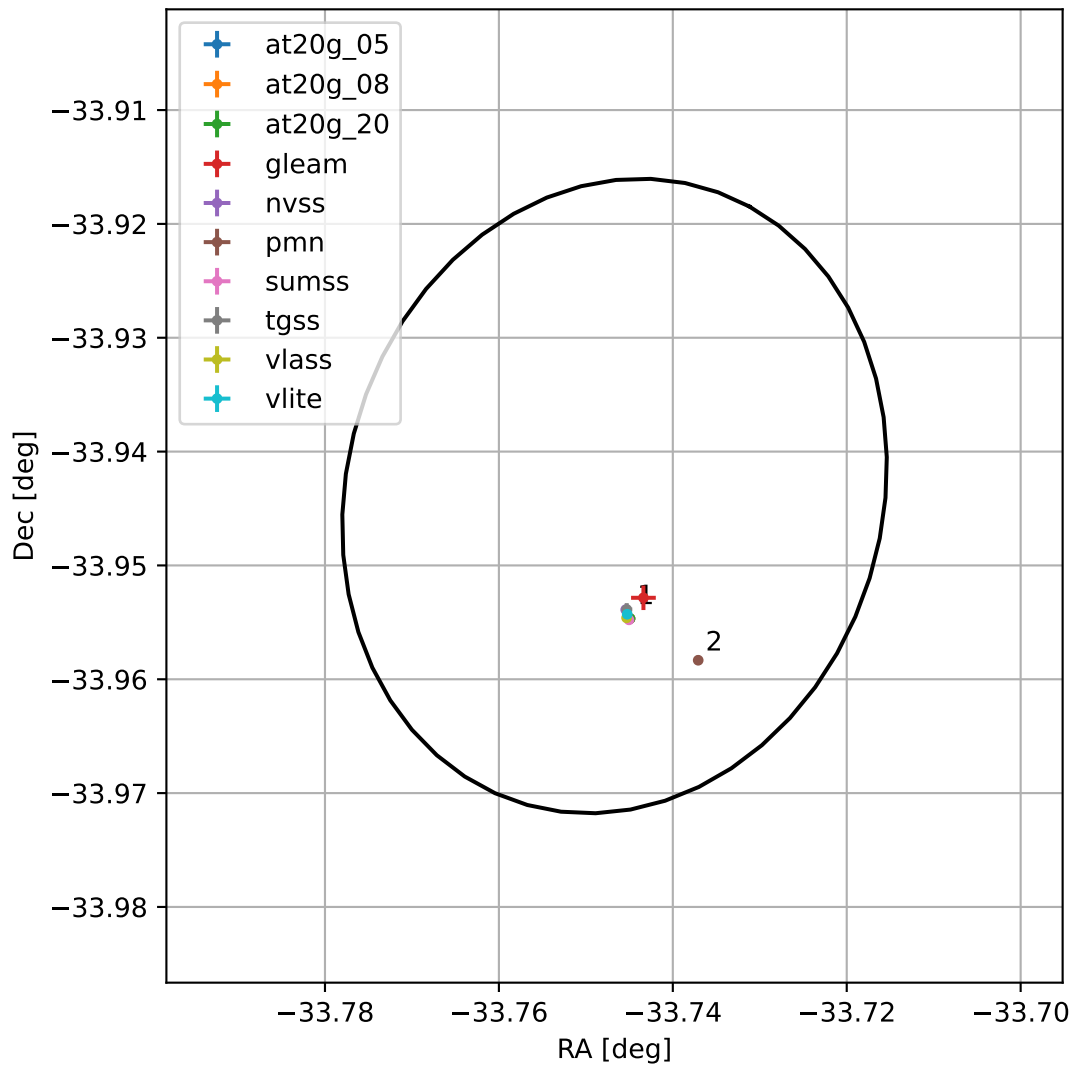
4FGL J2145.0-3356
