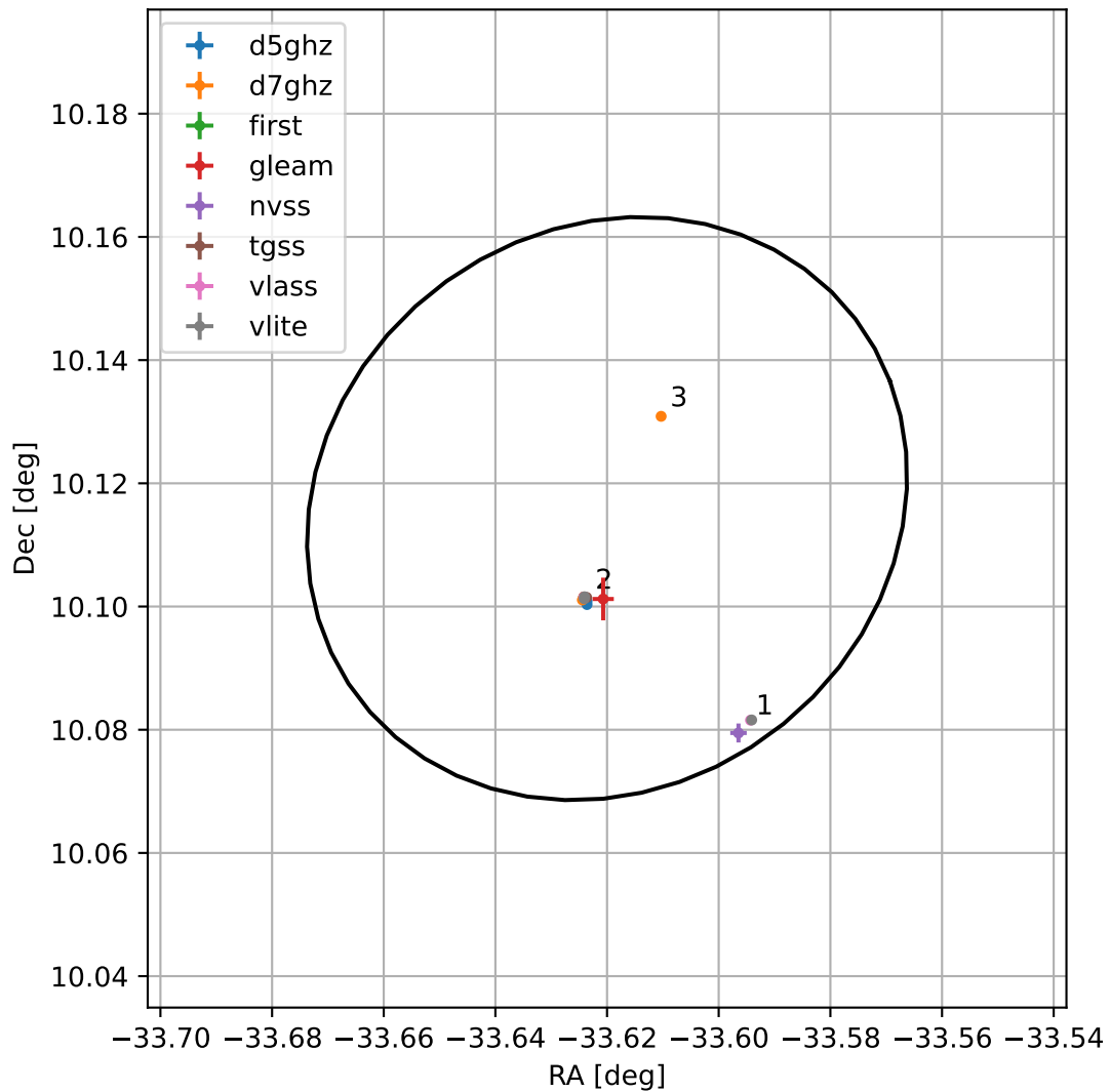
4FGL J2145.5+1006
